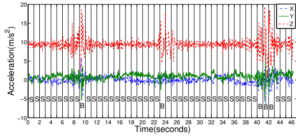
Fig. 5. Accelerometer Data for three speedbreakers
